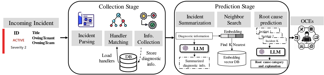
Figure 4. RCACOPILOT architecture.
